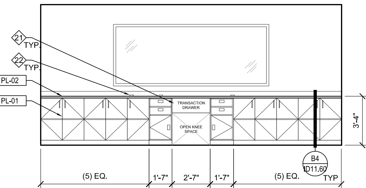
TELLER LINE 109
