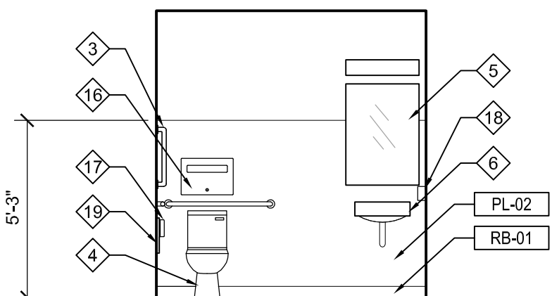
WOMEN'S RESTROOM 111 SCALE: 1/4"=1'-0"
